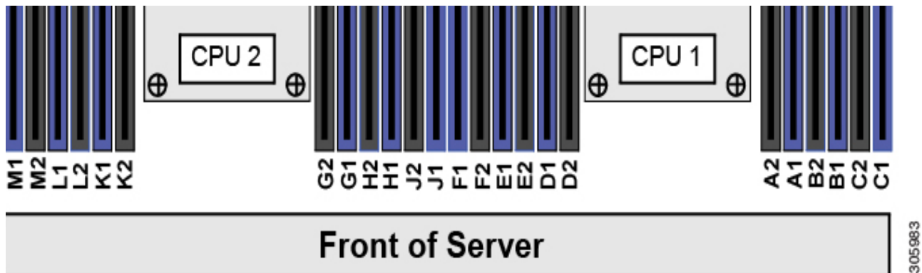
Figure 6 Figure: Physical Layout of CPU DIMM Channels and Slots
